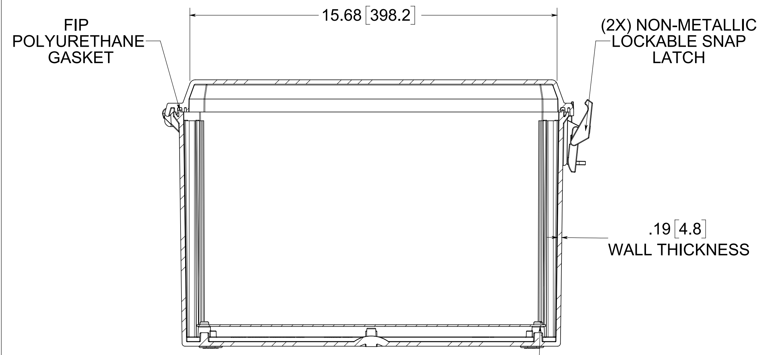
SECTION C-C
