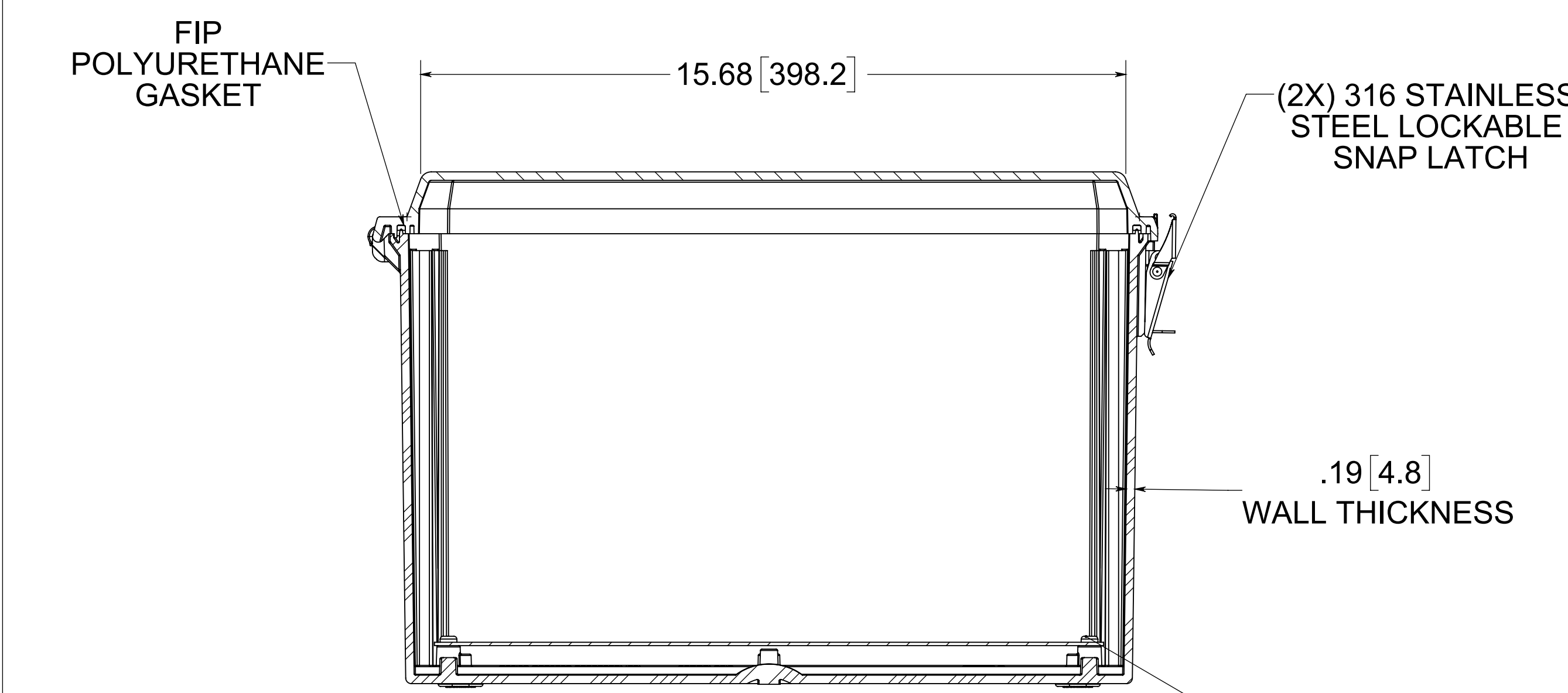
SECTION B-B
