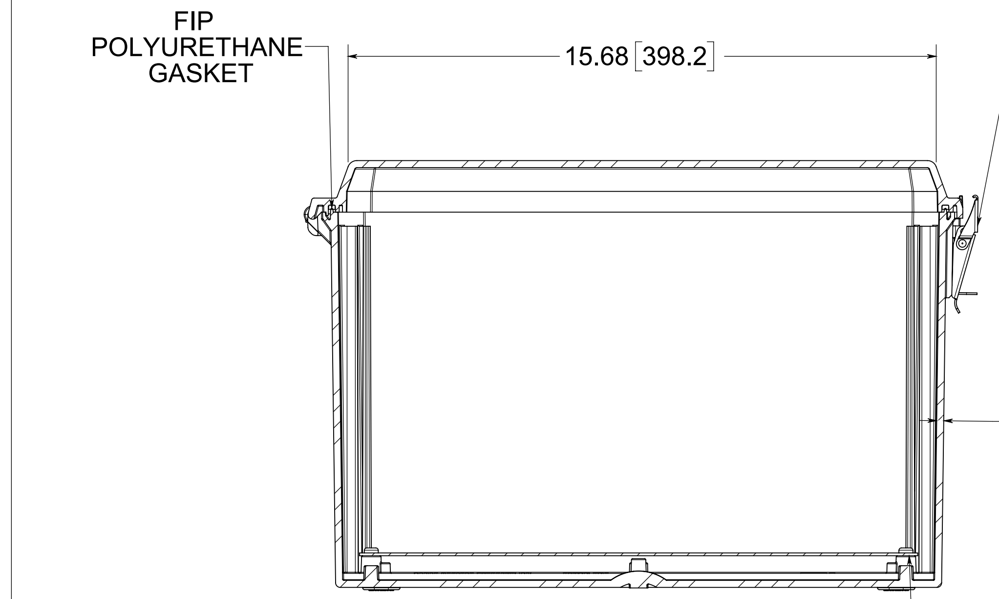
SECTION C-C
